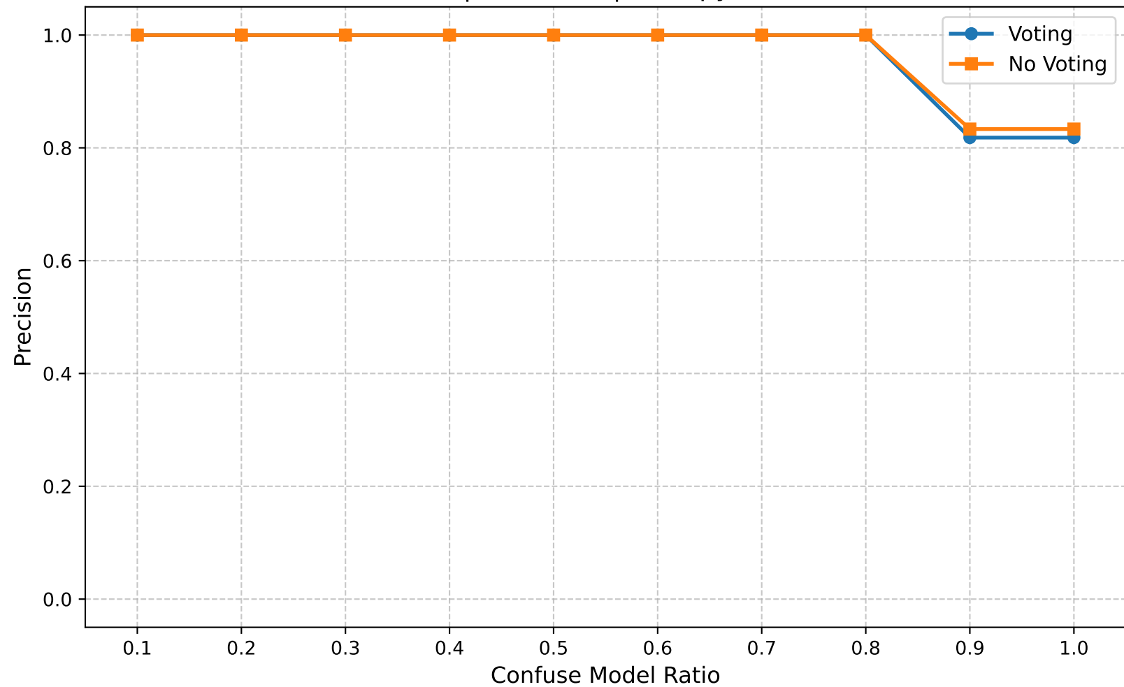
Precision | Round 10 | Entropy Ratio 0.55
