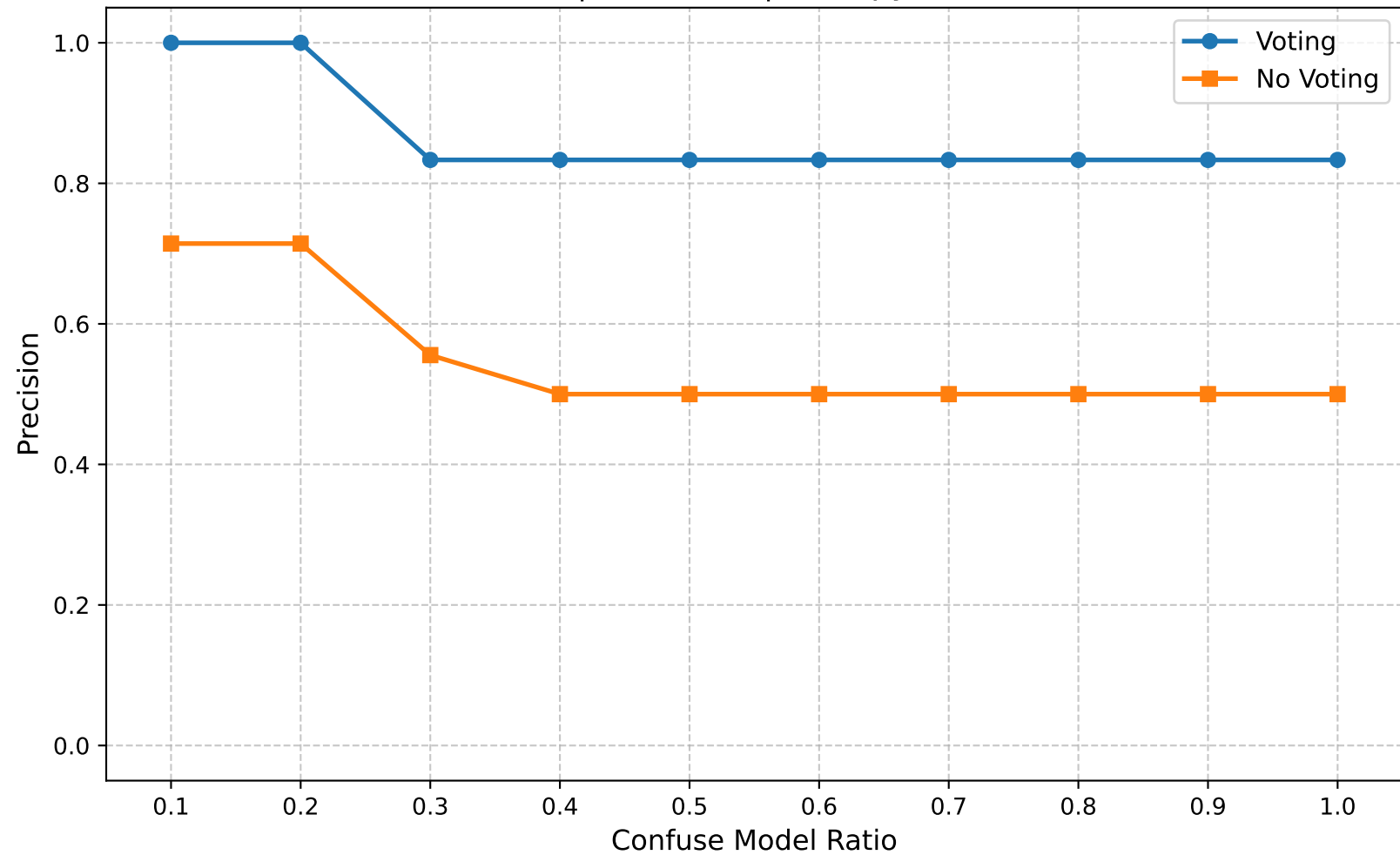
Precision | Round 10 | Entropy Ratio 0.95
