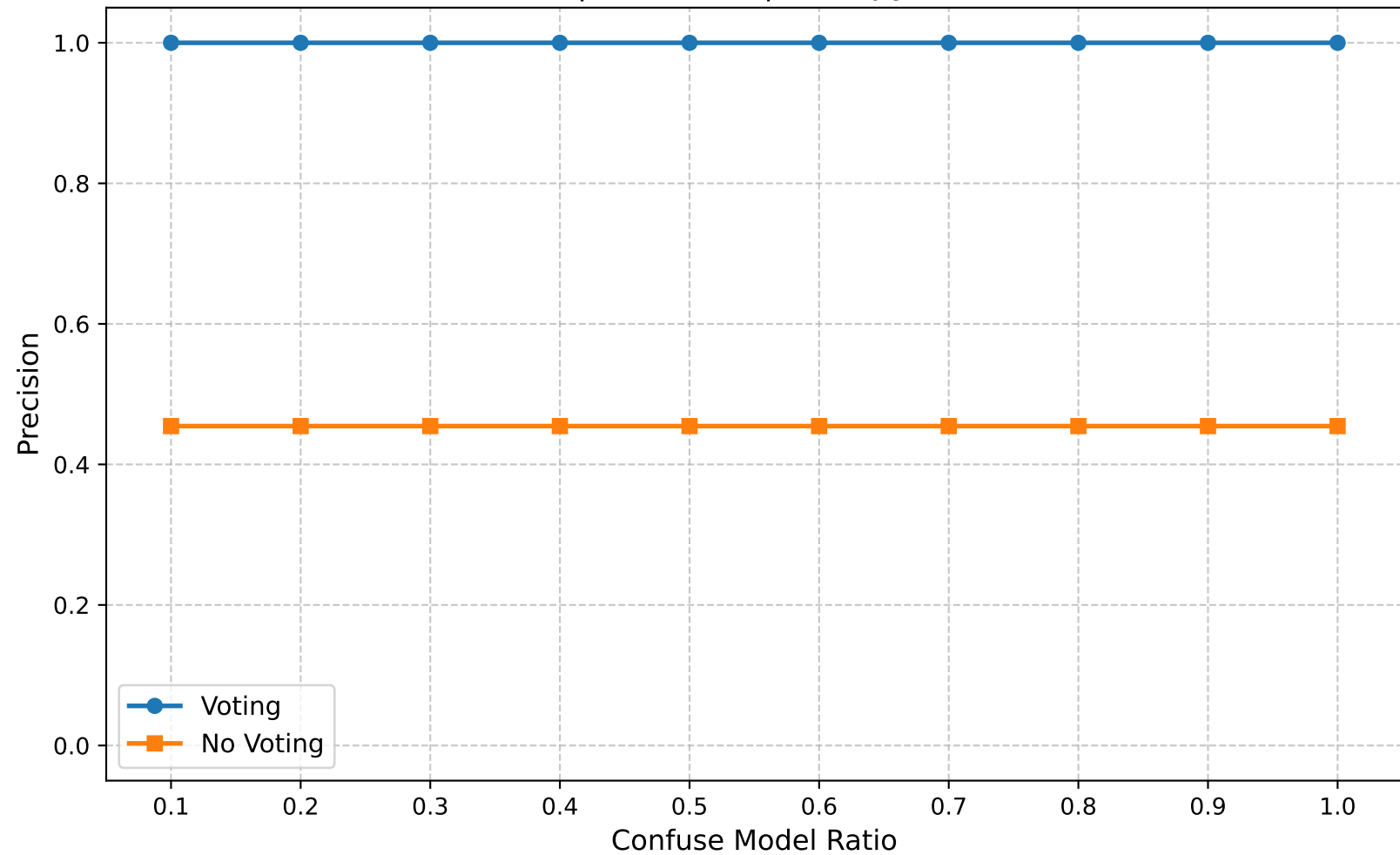
Precision | Round 10 | Entropy Ratio 1.00
