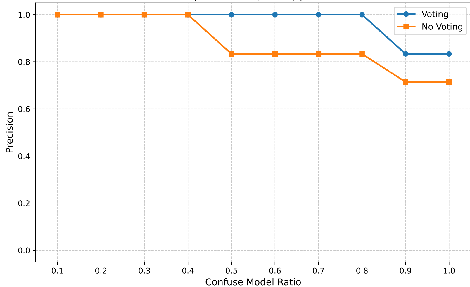
Precision | Round 15 | Entropy Ratio 0.55
