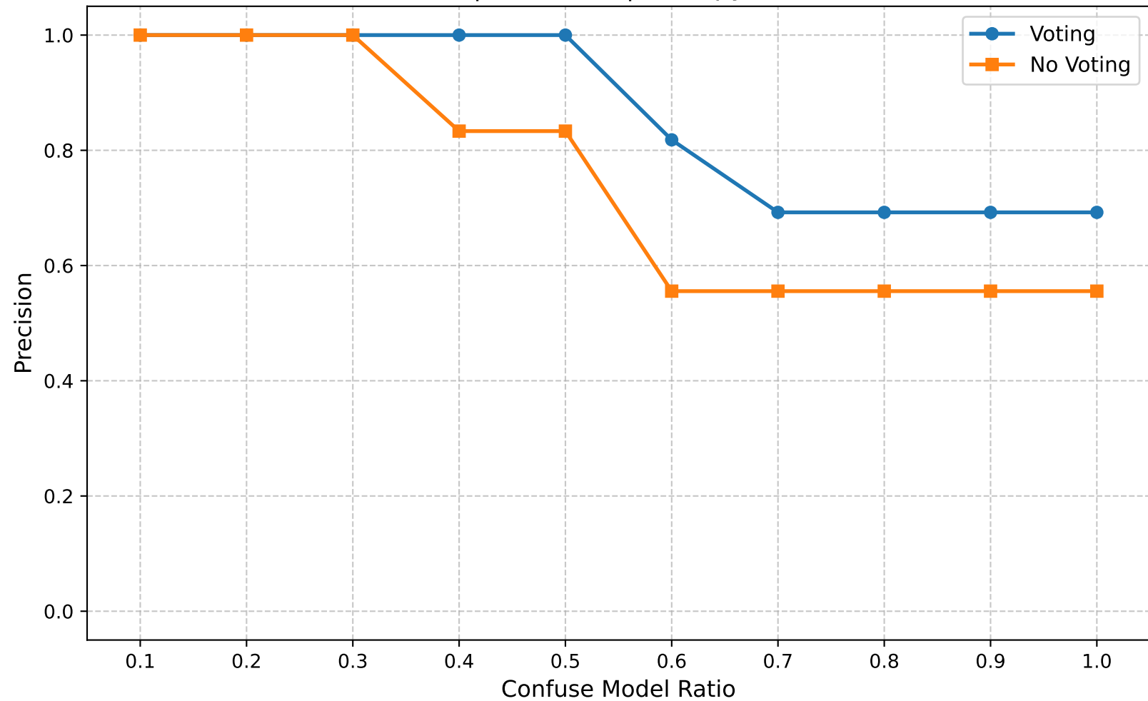
Precision | Round 15 | Entropy Ratio 0.80
