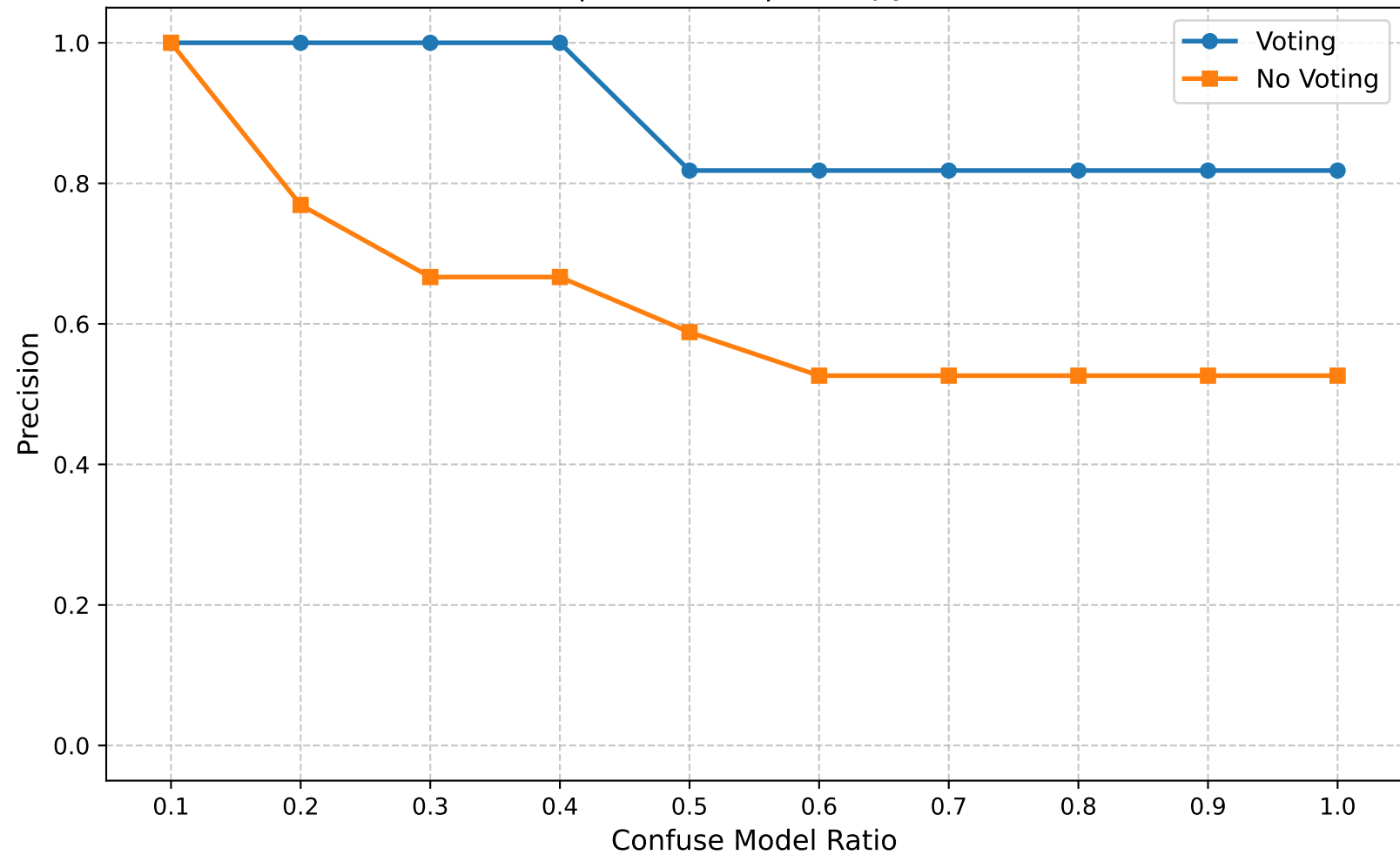
Precision | Round 15 | Entropy Ratio 0.85
