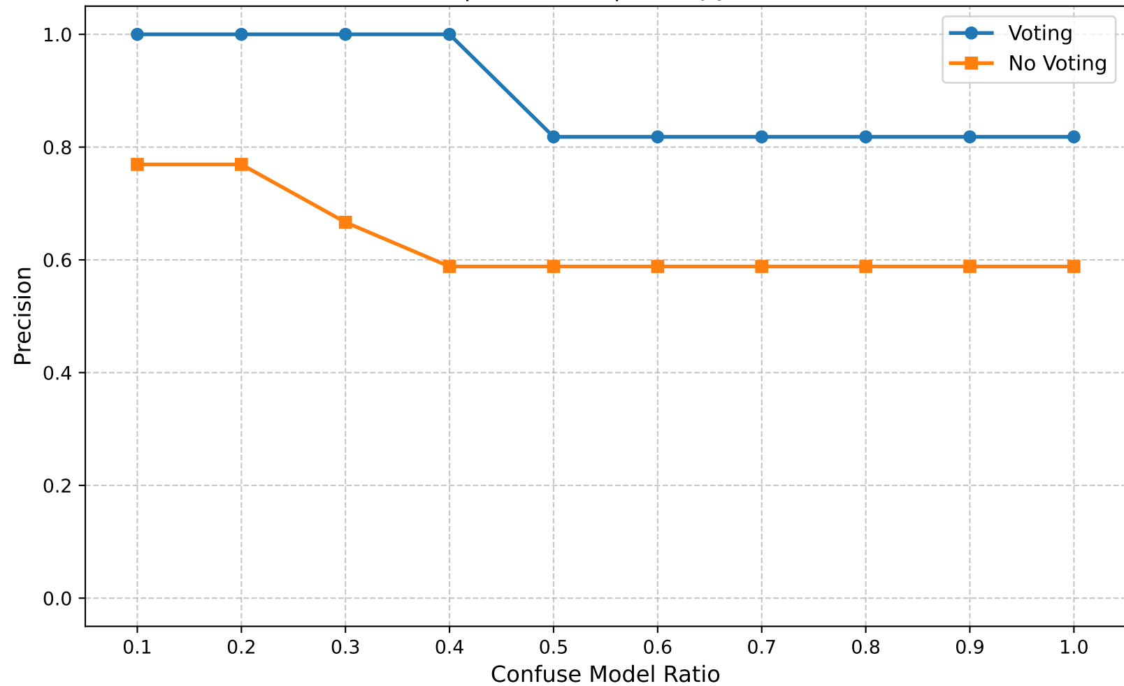
Precision | Round 15 | Entropy Ratio 0.90
