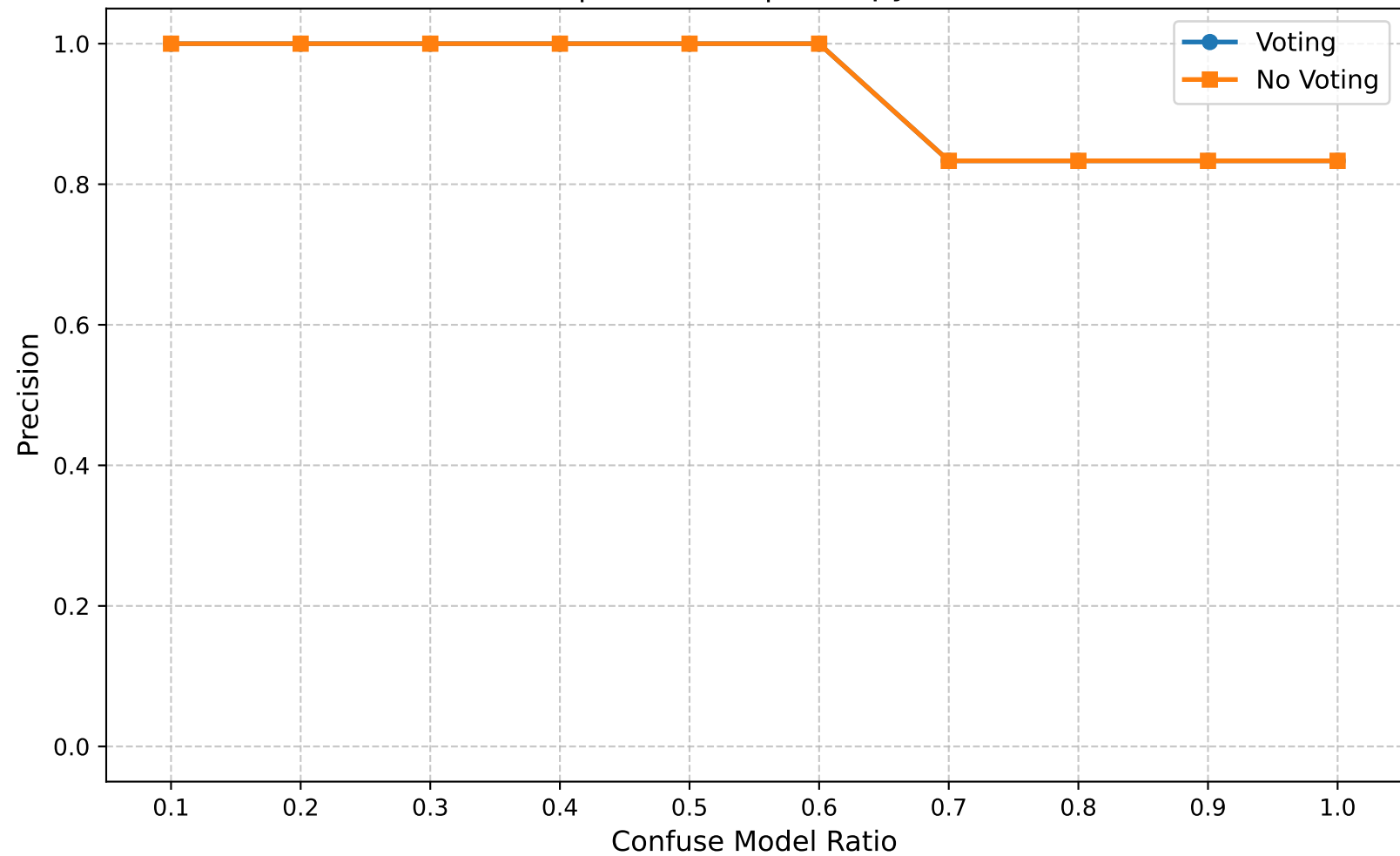
Precision | Round 20 | Entropy Ratio 0.45
