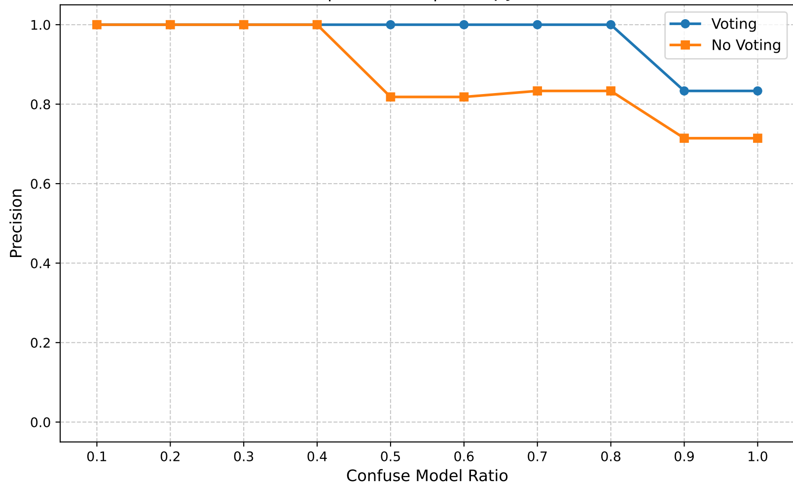
Precision | Round 20 | Entropy Ratio 0.55
