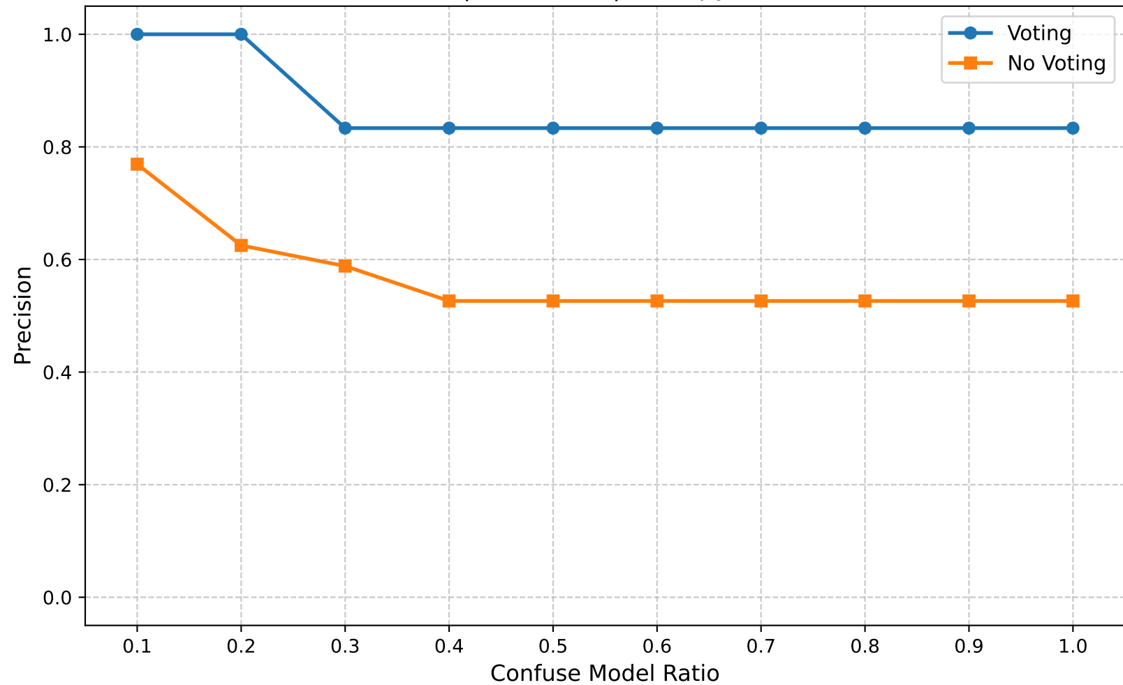
Precision | Round 20 | Entropy Ratio 0.95
