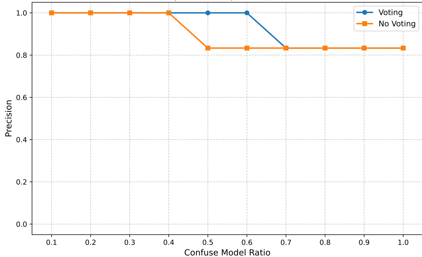
Precision | Round 25 | Entropy Ratio 0.45
