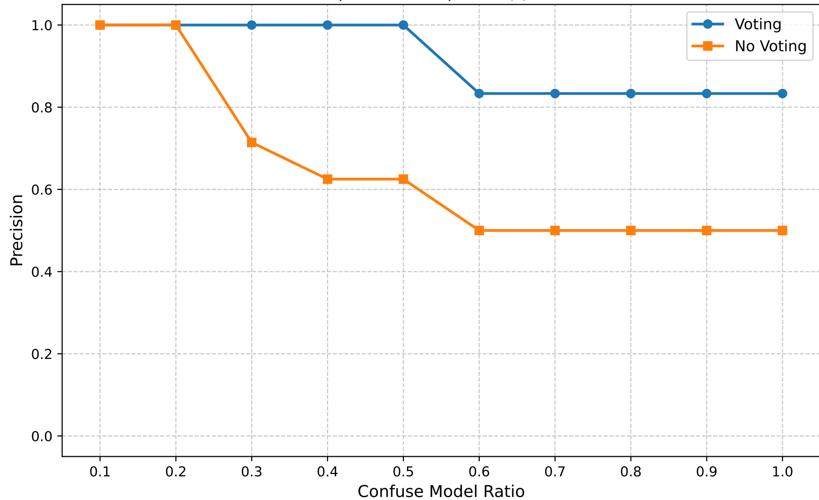
Precision | Round 25 | Entropy Ratio 0.80
