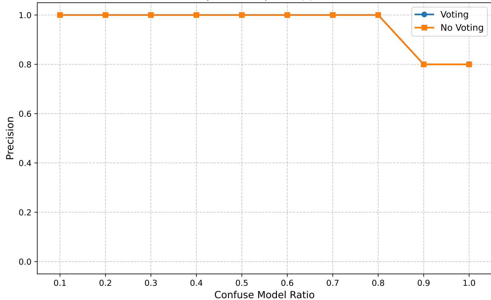
Precision | Round 5 | Entropy Ratio 0.25
