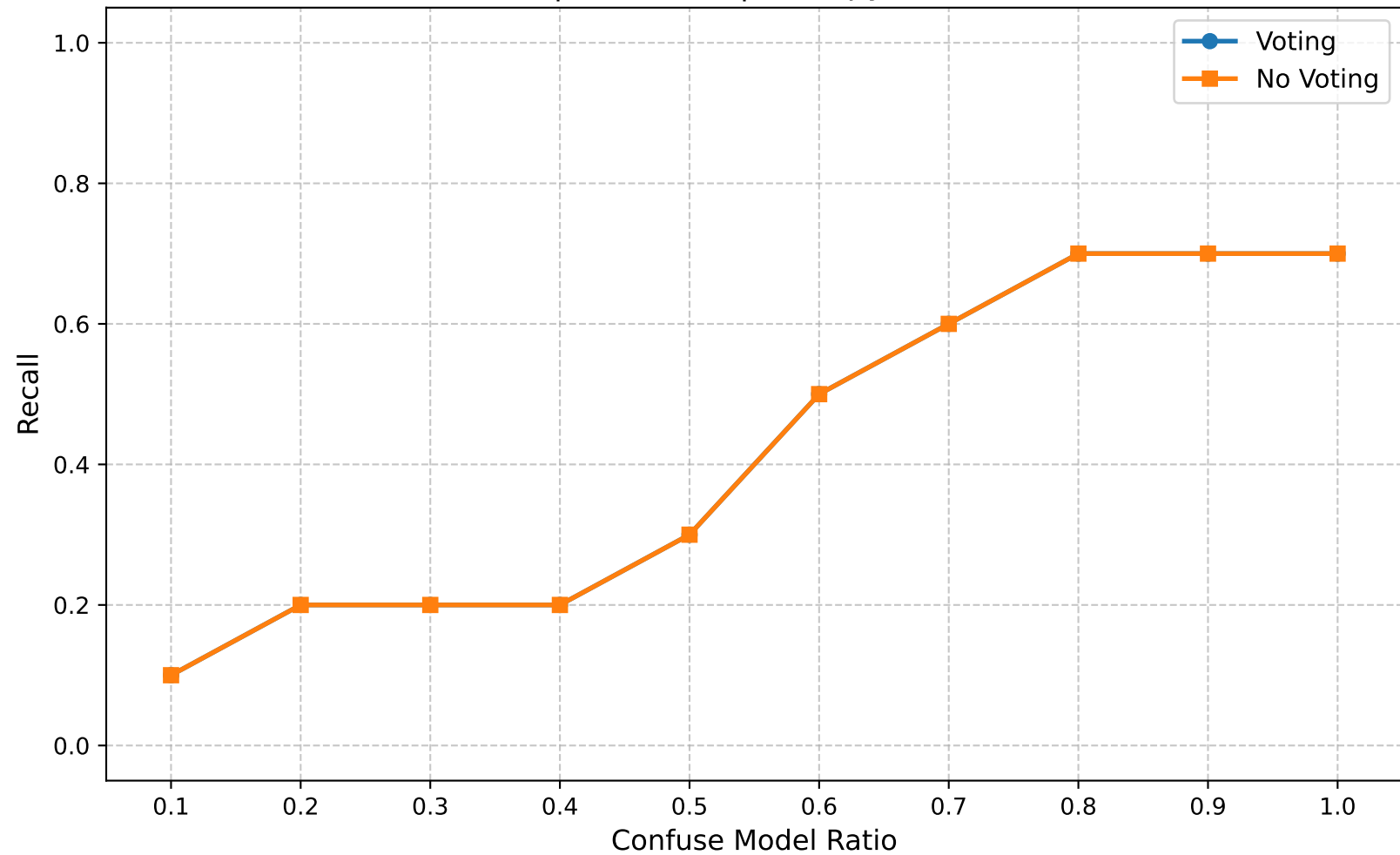
Recall | Round 10 | Entropy Ratio 0.25
