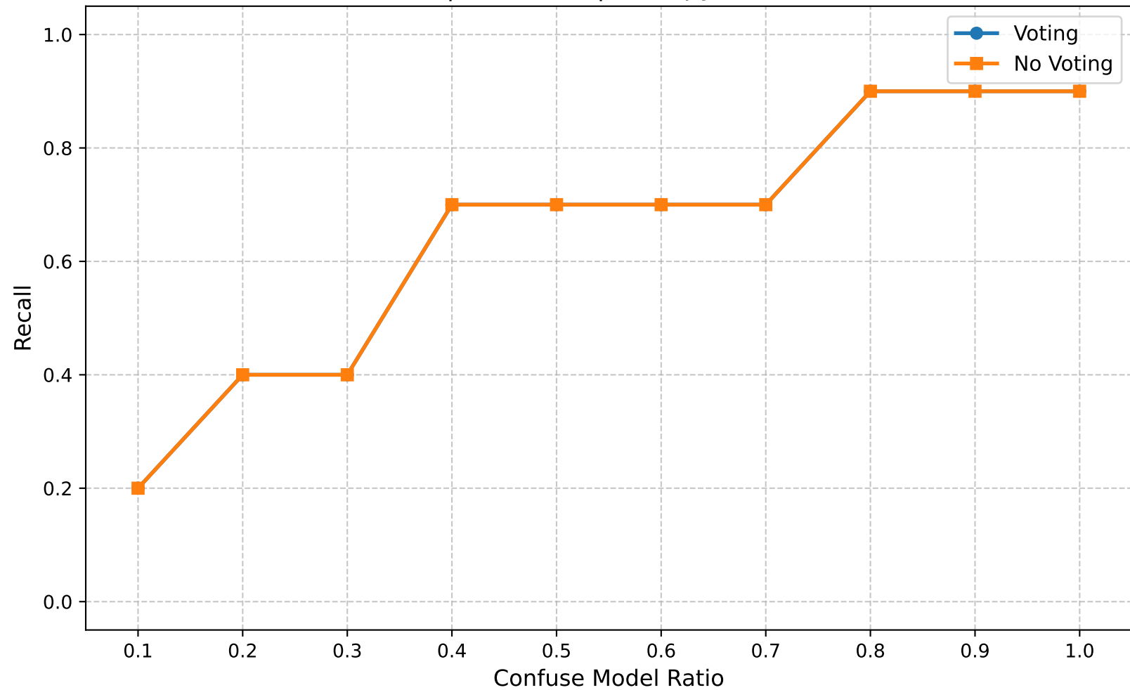
Recall | Round 10 | Entropy Ratio 0.35
