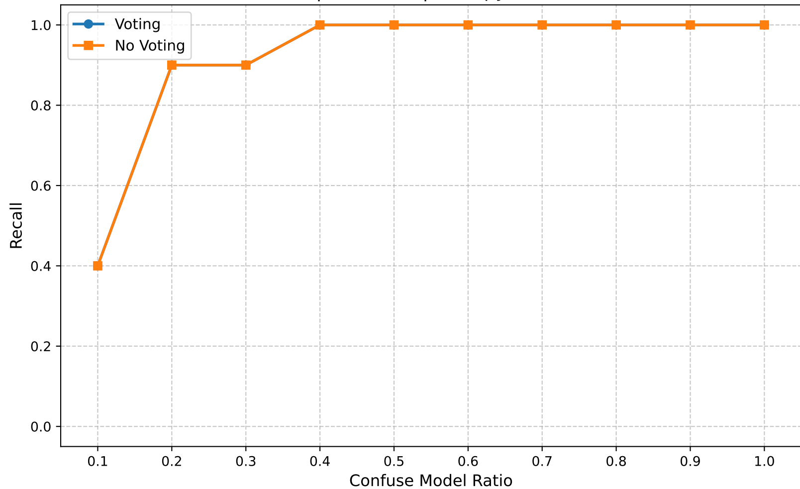
Recall | Round 15 | Entropy Ratio 0.50
