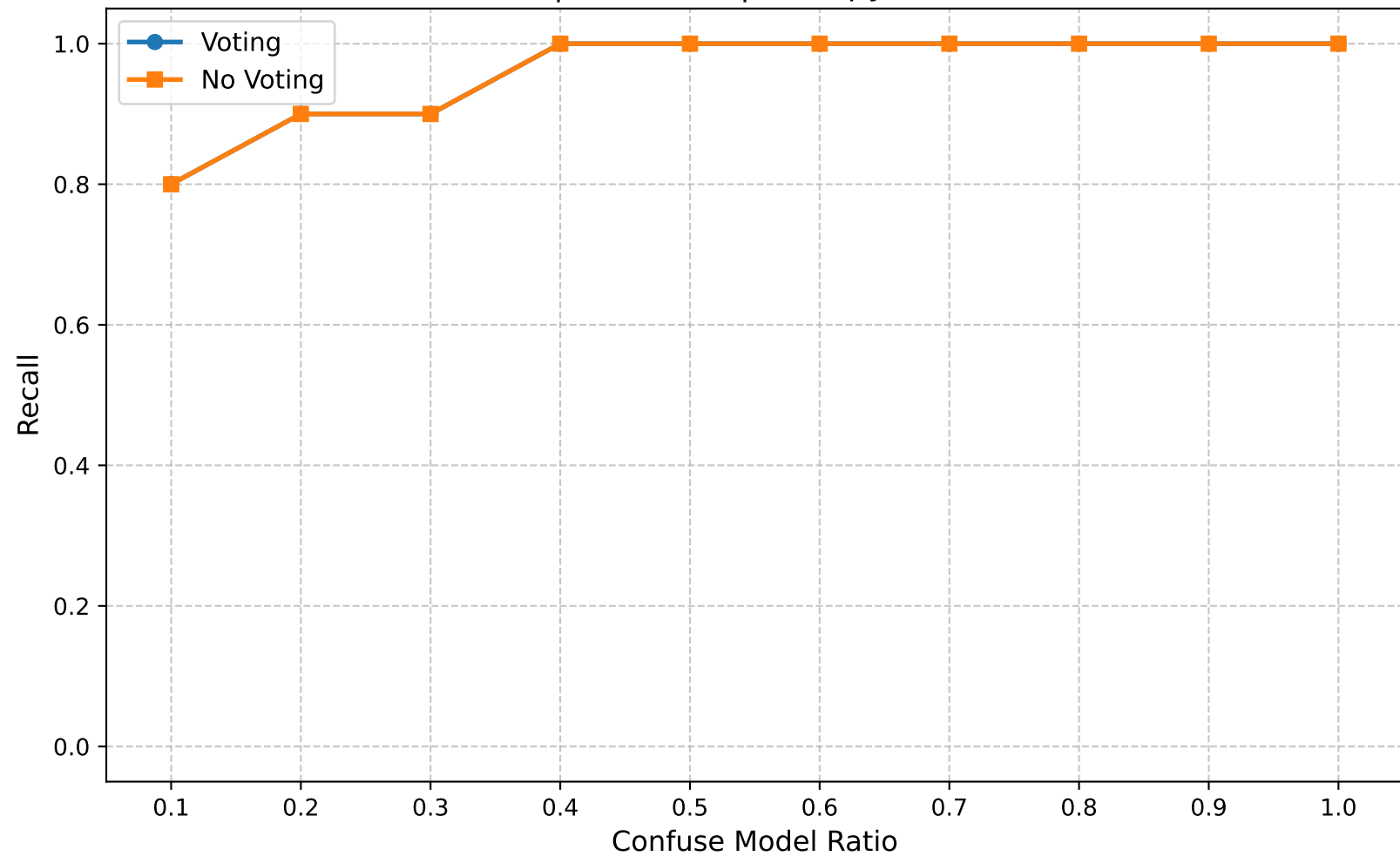
Recall | Round 15 | Entropy Ratio 0.55
