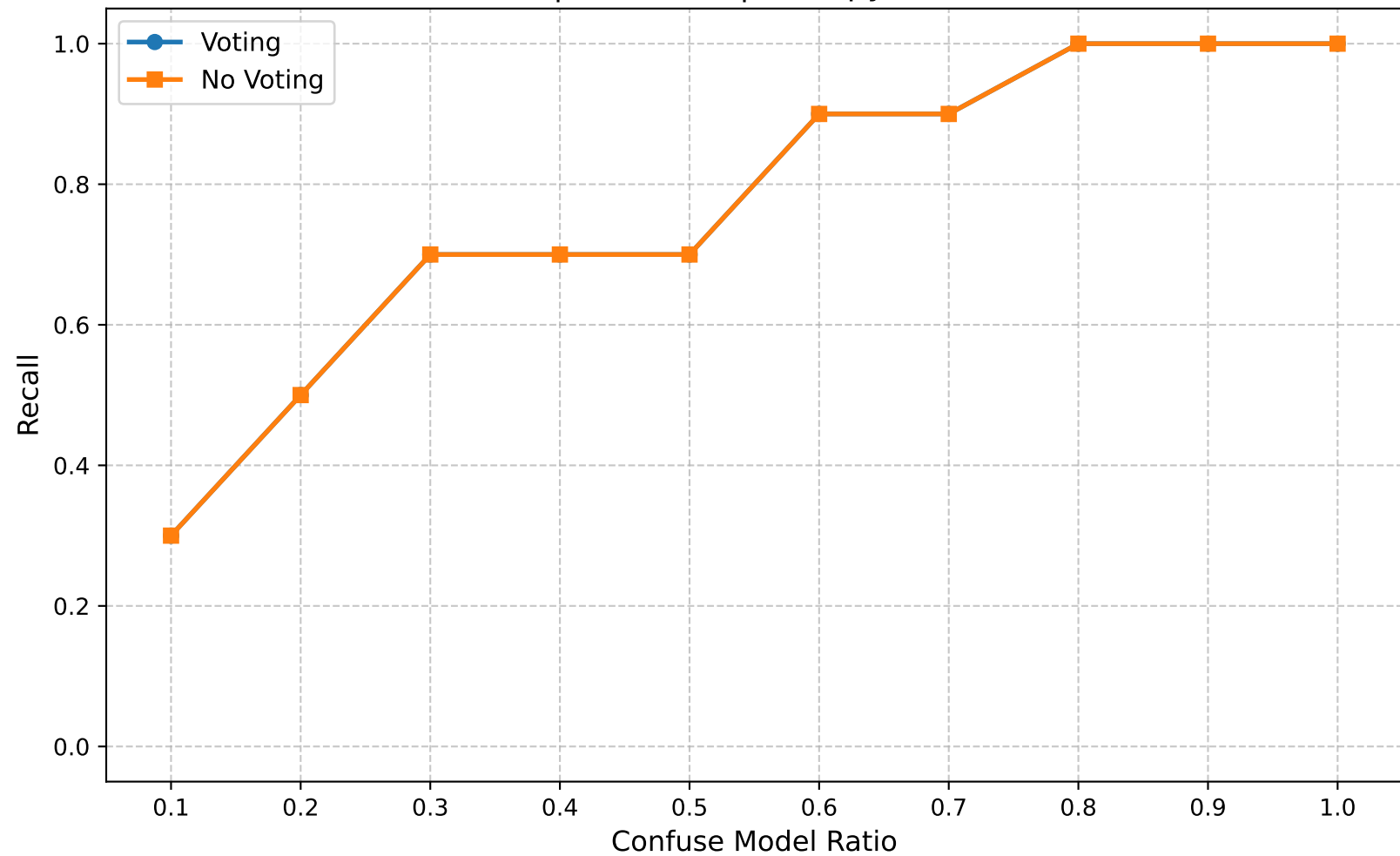
Recall | Round 20 | Entropy Ratio 0.40
