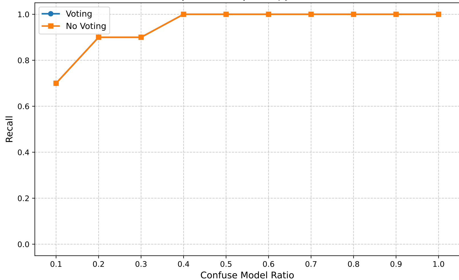
Recall | Round 20 | Entropy Ratio 0.65
