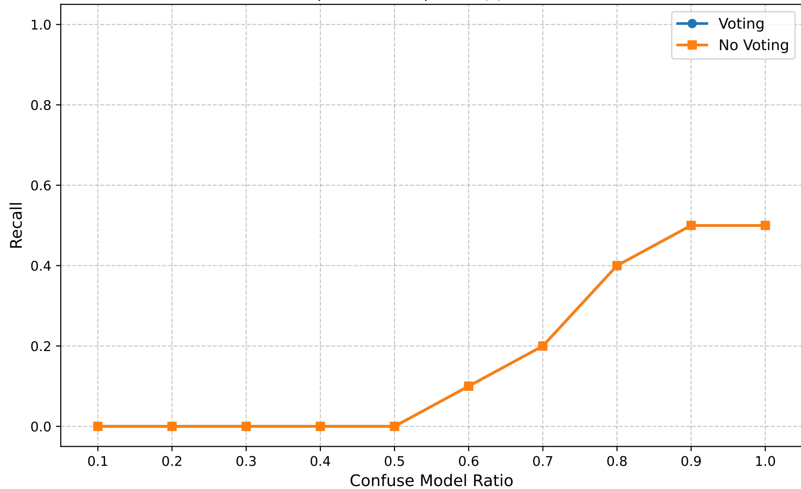
Recall | Round 25 | Entropy Ratio 0.10
