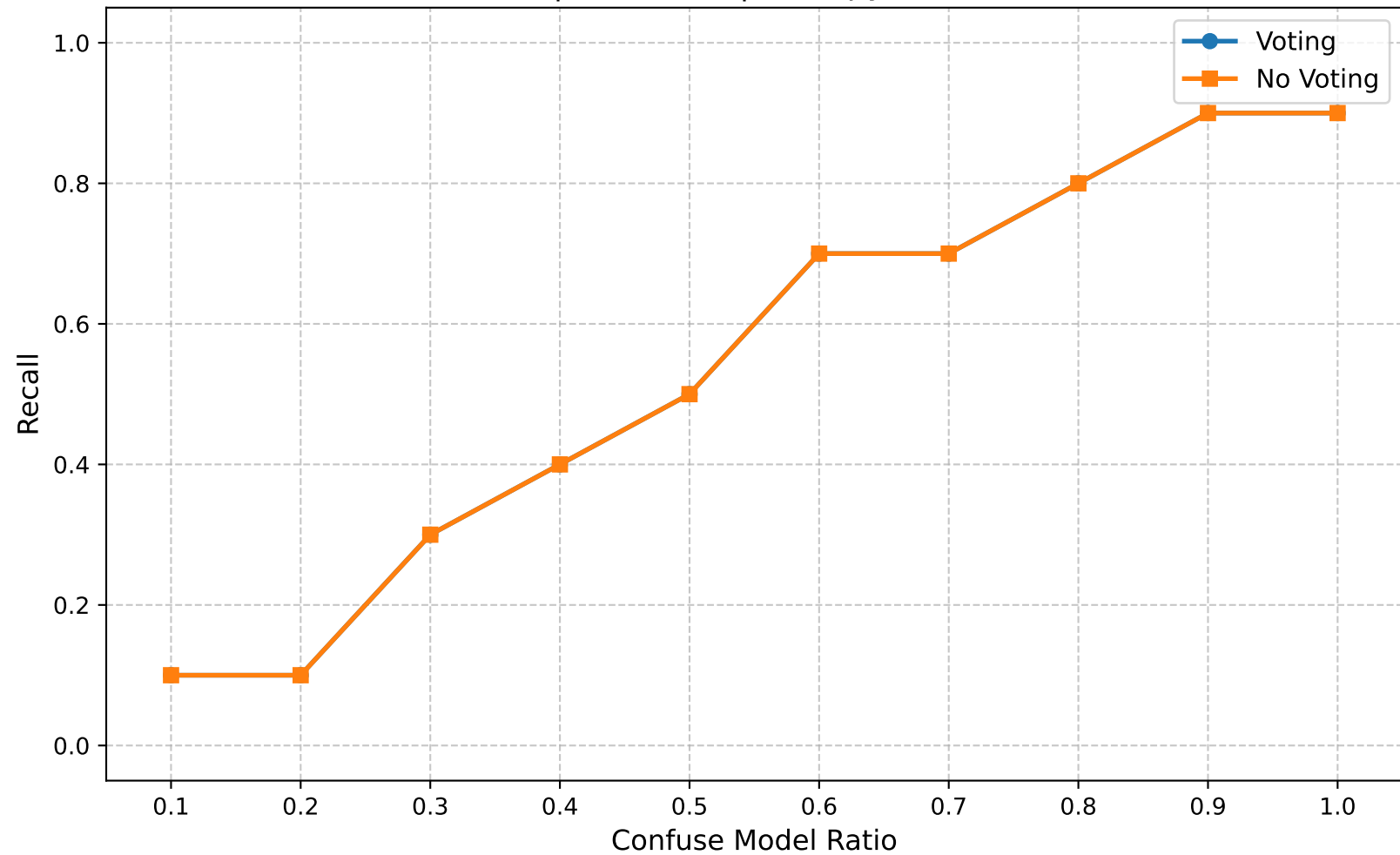
Recall | Round 25 | Entropy Ratio 0.30
