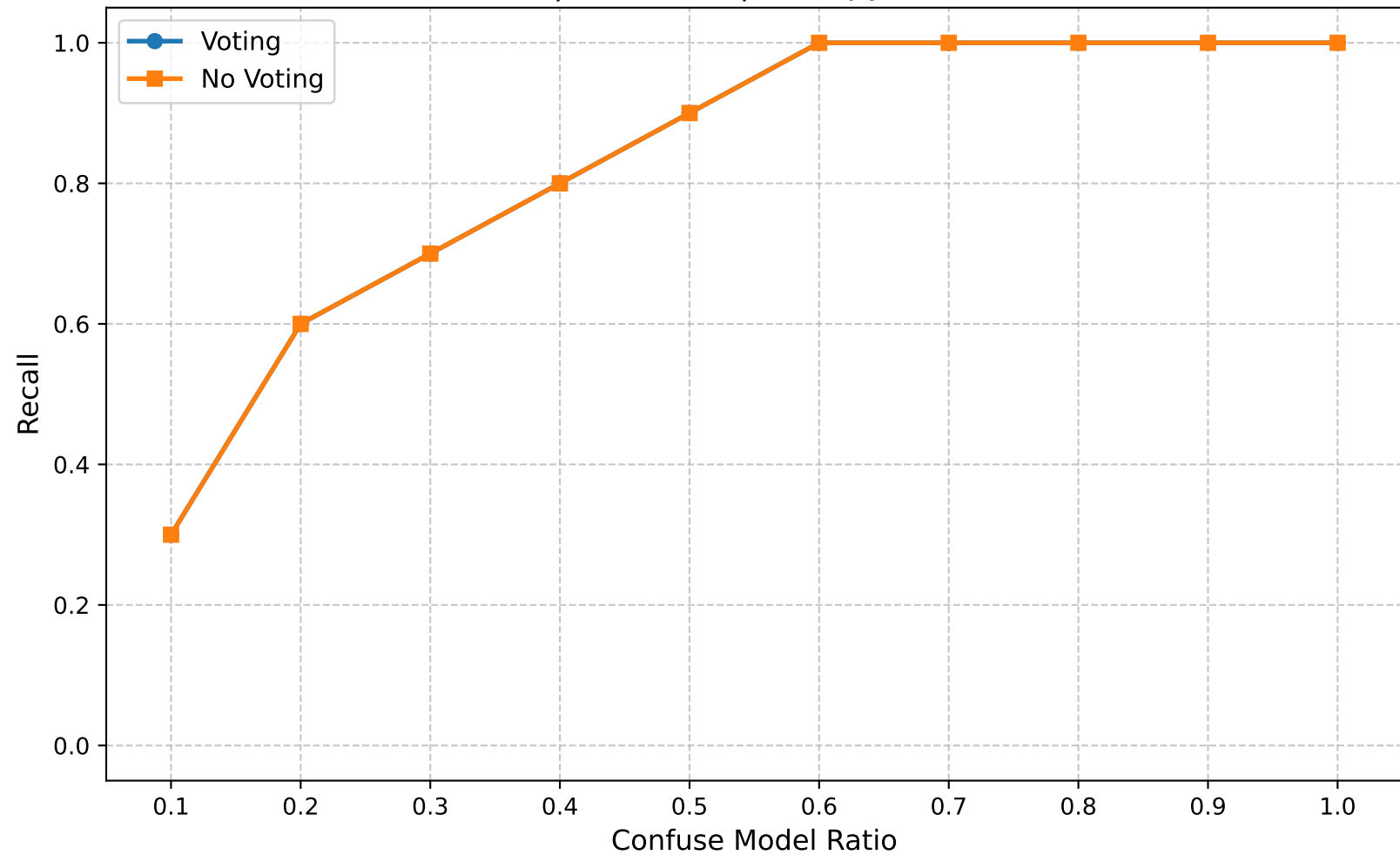
Recall | Round 25 | Entropy Ratio 0.40
