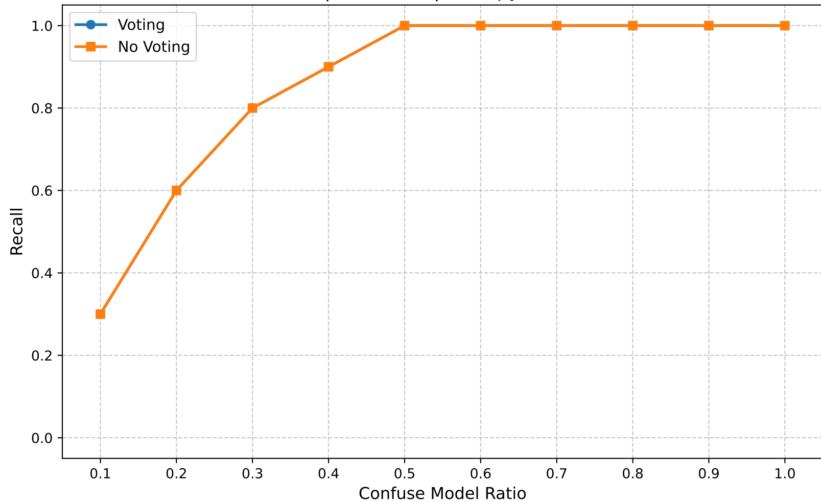
Recall | Round 25 | Entropy Ratio 0.45
