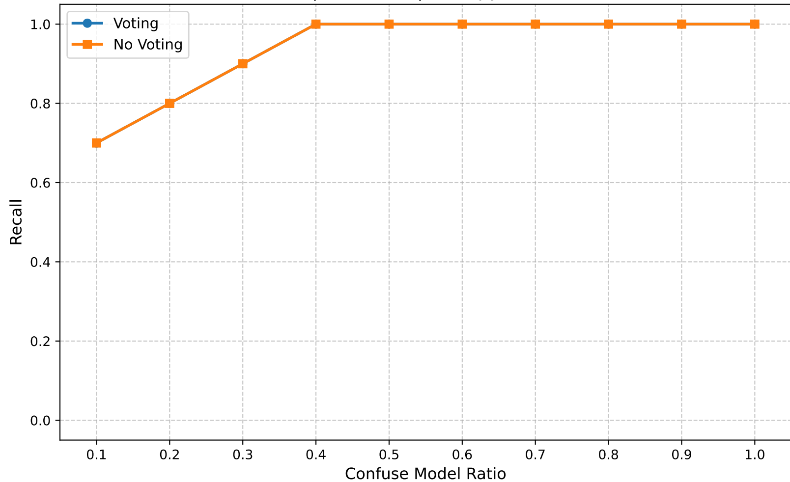
Recall | Round 25 | Entropy Ratio 0.60
