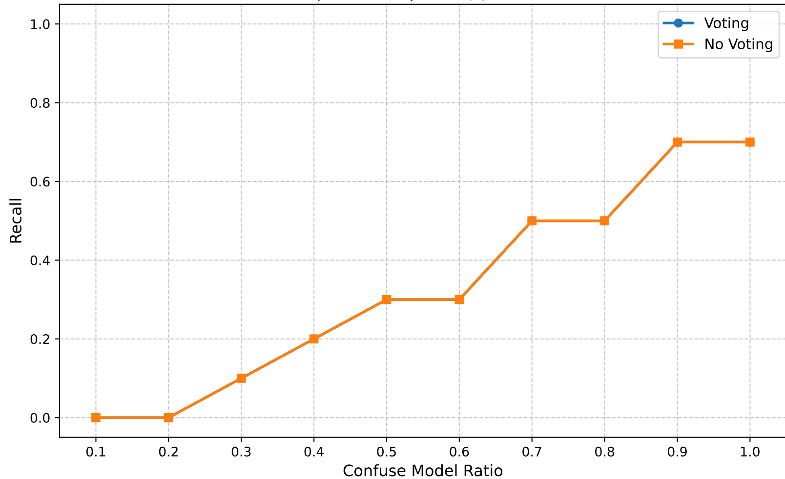
Recall | Round 5 | Entropy Ratio 0.15
