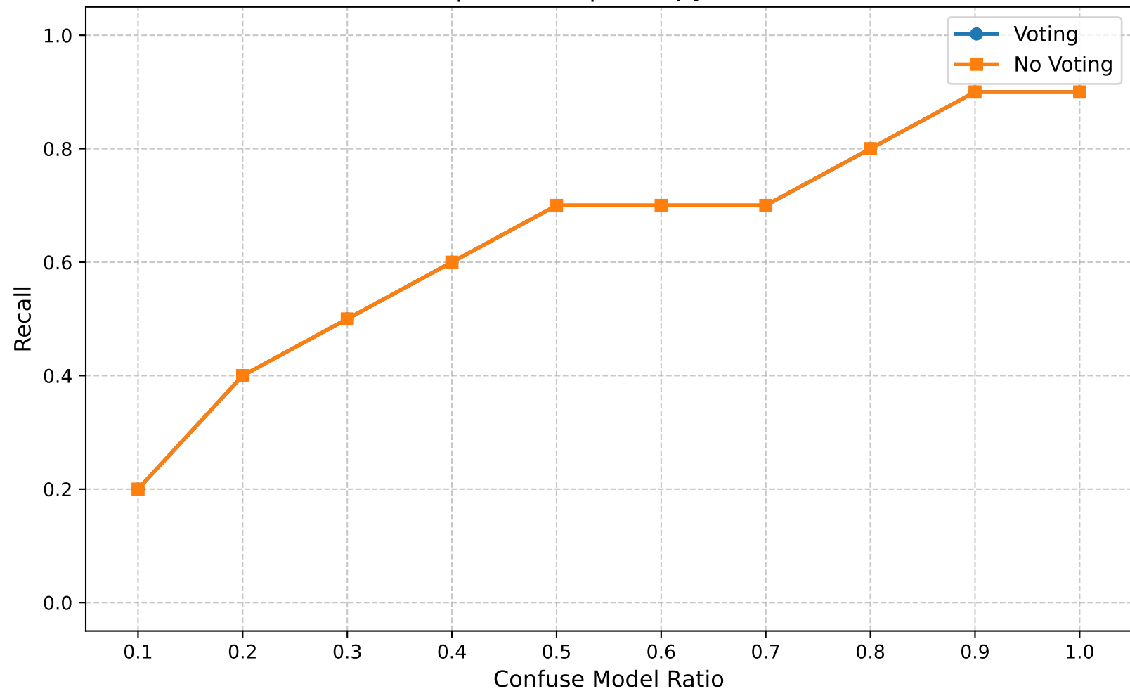
Recall | Round 5 | Entropy Ratio 0.30
