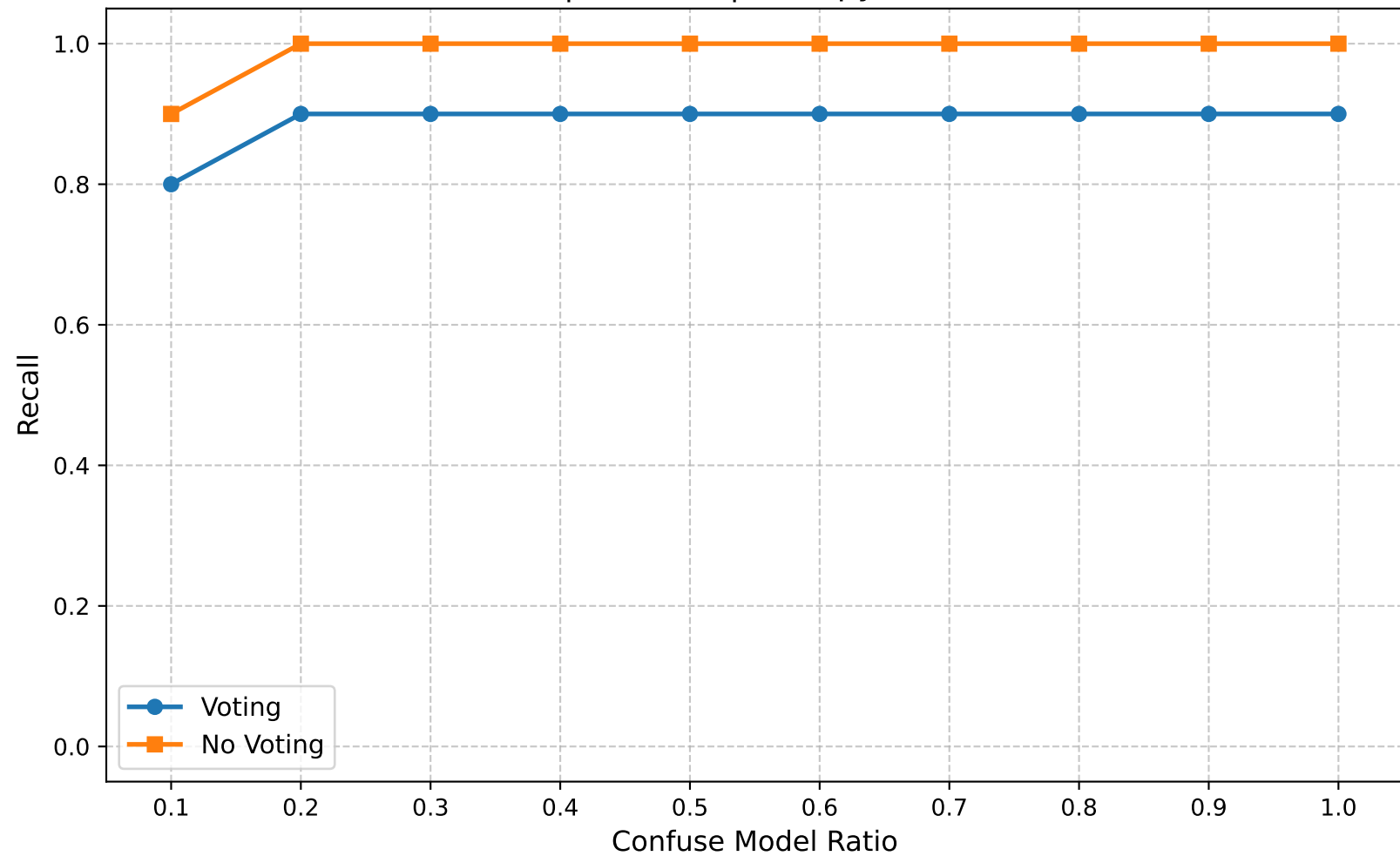
Recall | Round 5 | Entropy Ratio 0.65
