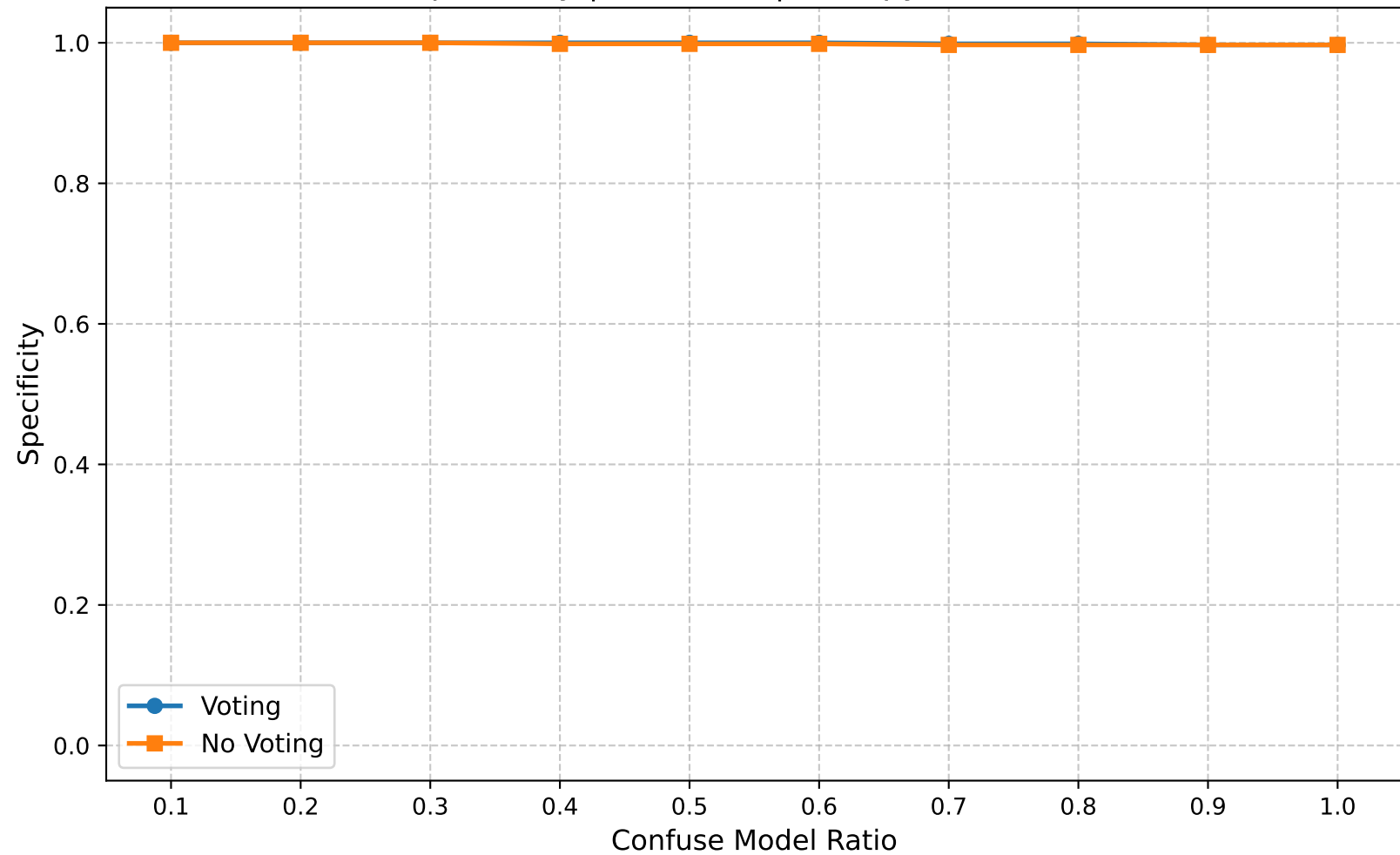
Specificity | Round 15 | Entropy Ratio 0.70
