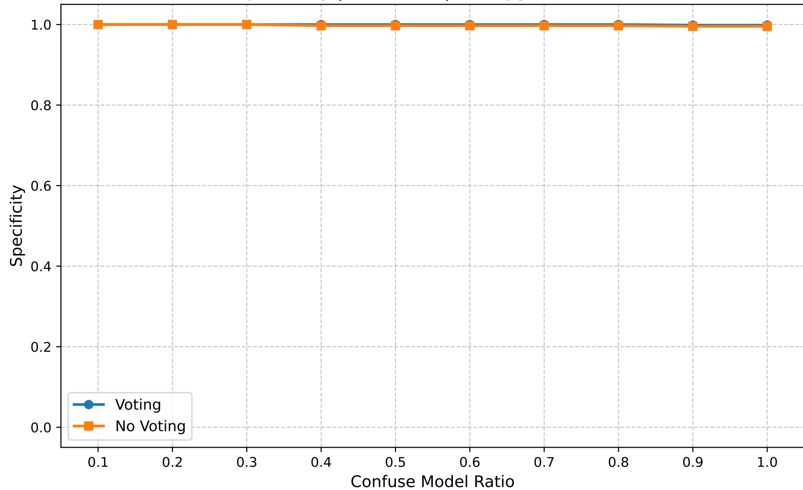
Specificity | Round 25 | Entropy Ratio 0.65
