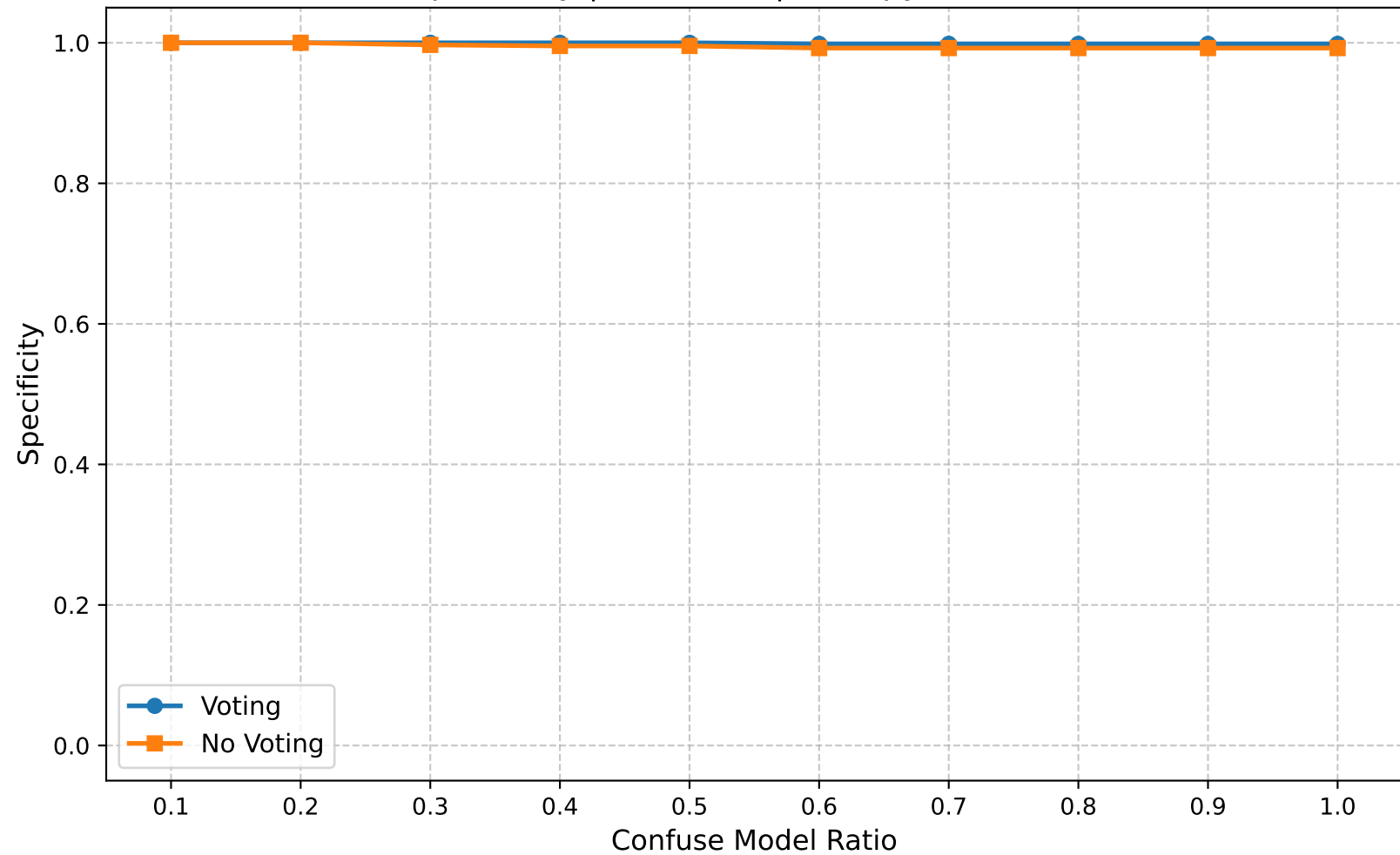
Specificity | Round 25 | Entropy Ratio 0.80
