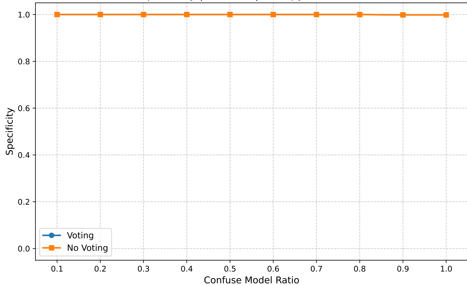
Specificity | Round 5 | Entropy Ratio 0.10
