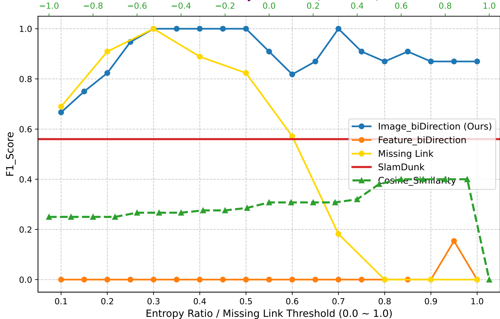
F1_Score (Global Round: 5) Cosine Similarity Threshold (-1.0 ~ 1.0)
