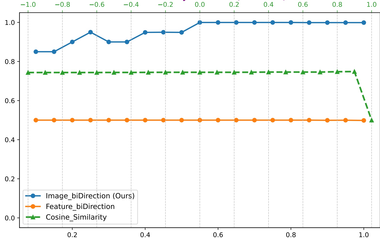
Average_Accuracy (Global Round: 10) Cosine Similarity Threshold (-1.0 ~ 1.0)
