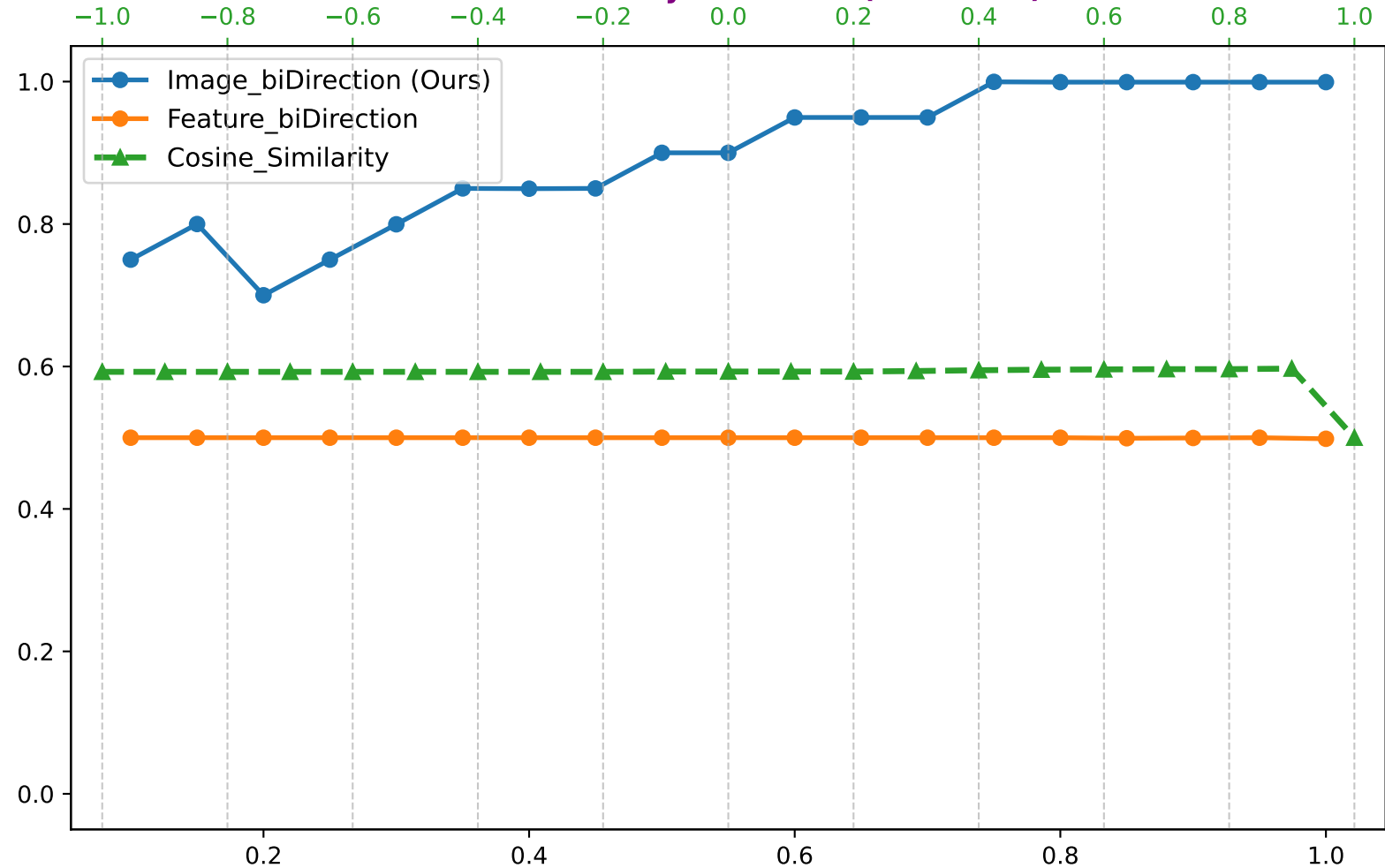
Average_Accuracy (Global Round: 20) Cosine Similarity Threshold (-1.0 ~ 1.0)
