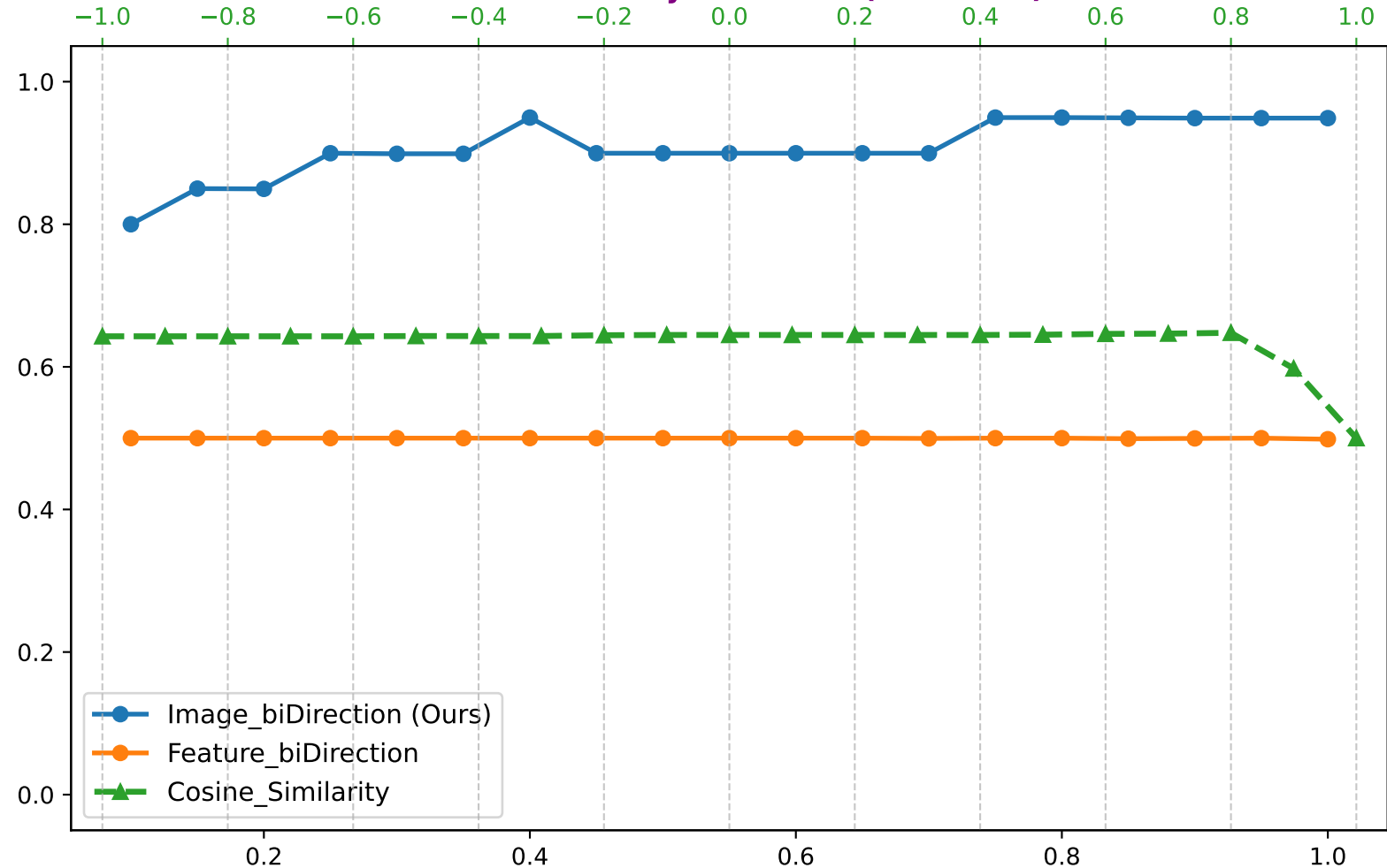
Average_Accuracy (Global Round: 40) Cosine Similarity Threshold (-1.0 ~ 1.0)
