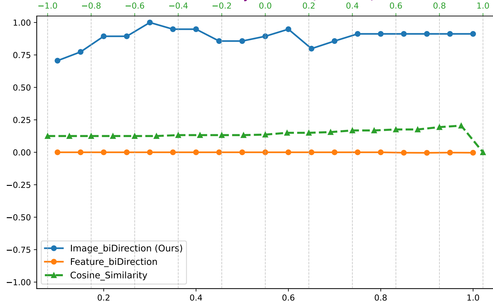
MCC (Global Round: 15) Cosine Similarity Threshold (-1.0 ~ 1.0)
