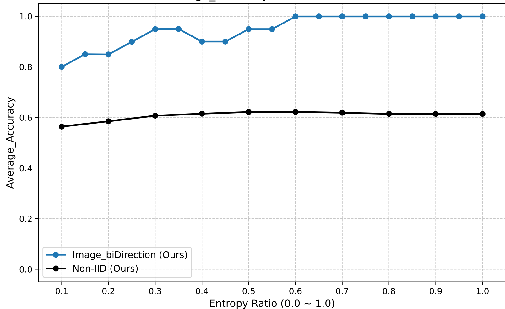
Average_Accuracy (Global Round: 30)
