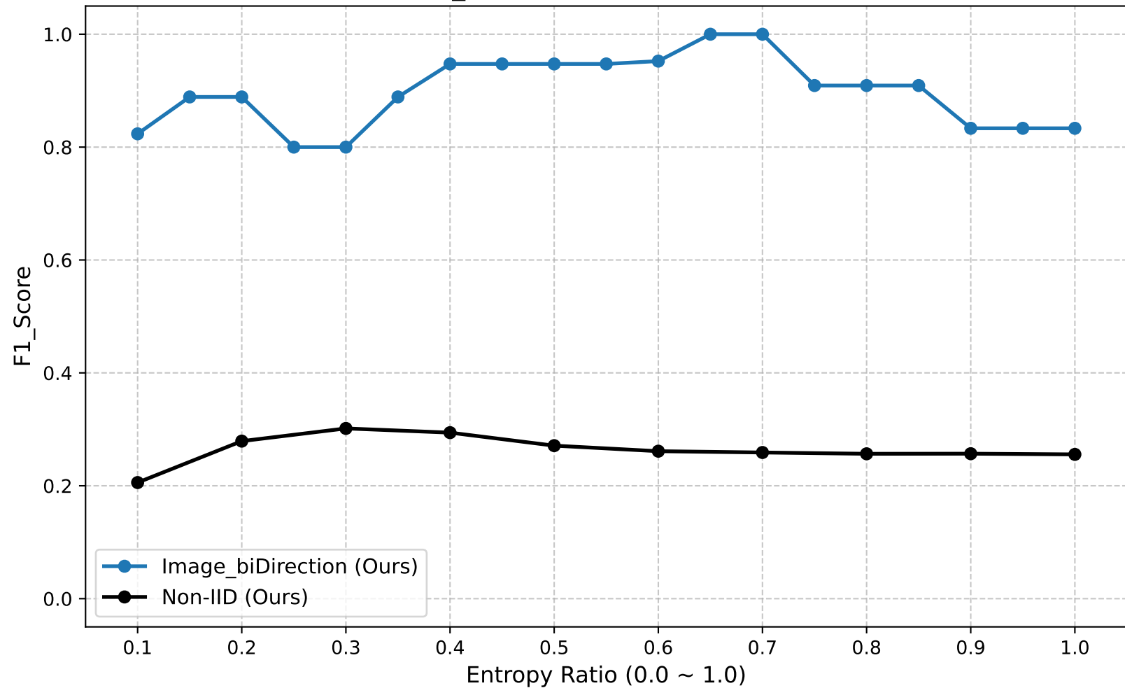
F1_Score (Global Round: 35)
