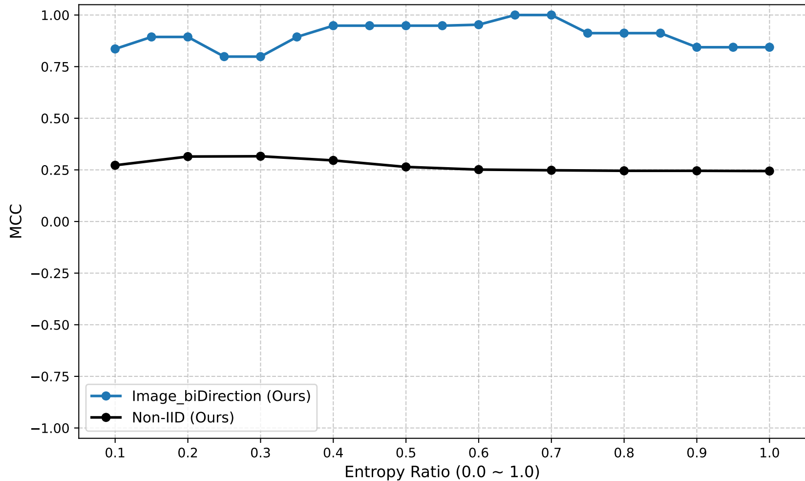
MCC (Global Round: 35)
