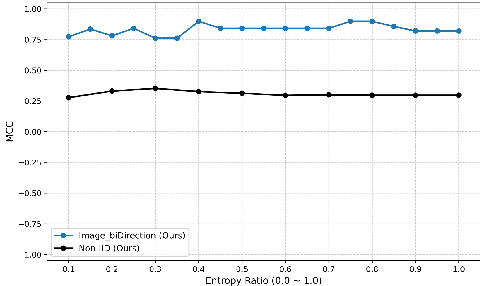
MCC (Global Round: 40)
