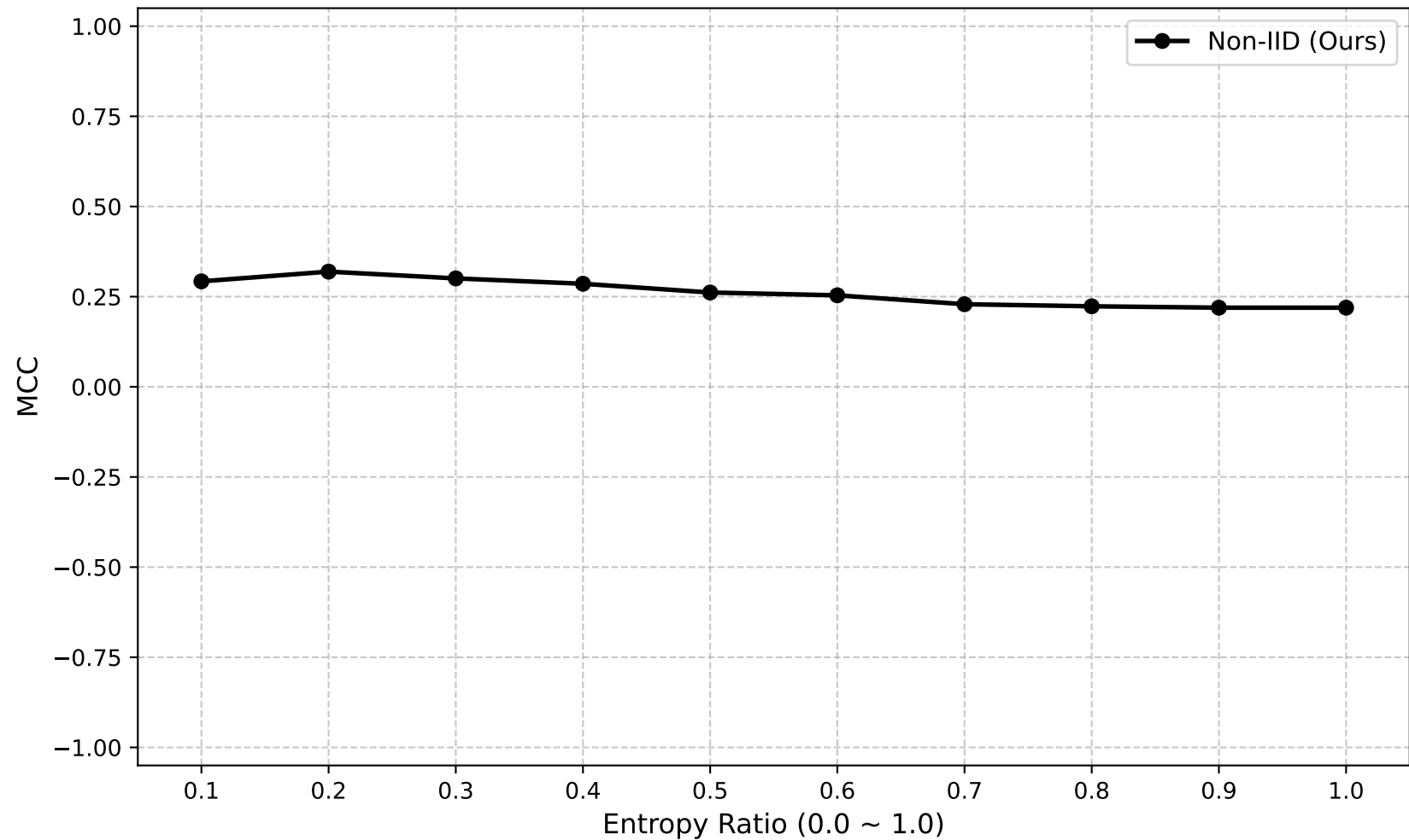
MCC (Global Round: 50)
