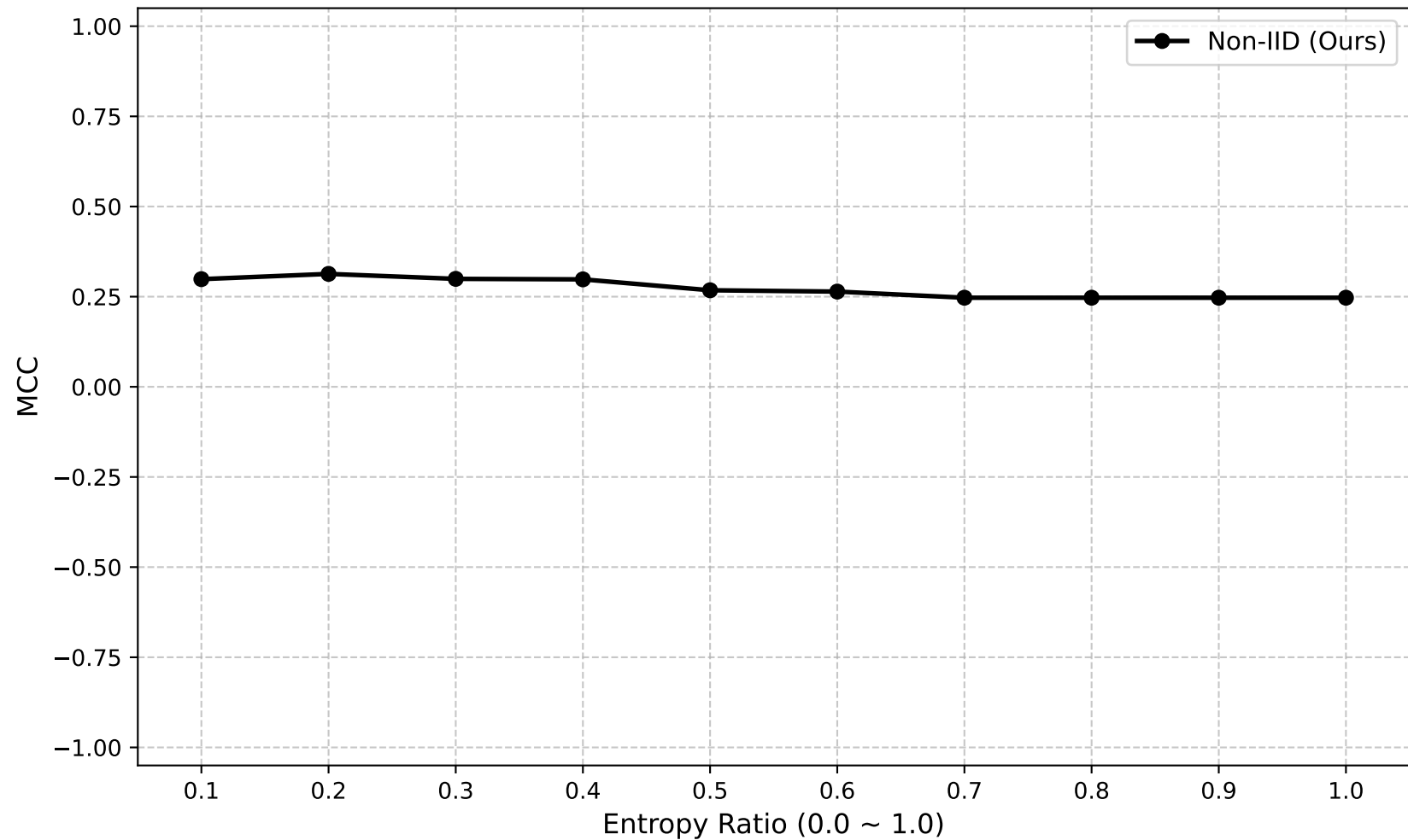
MCC (Global Round: 60)
