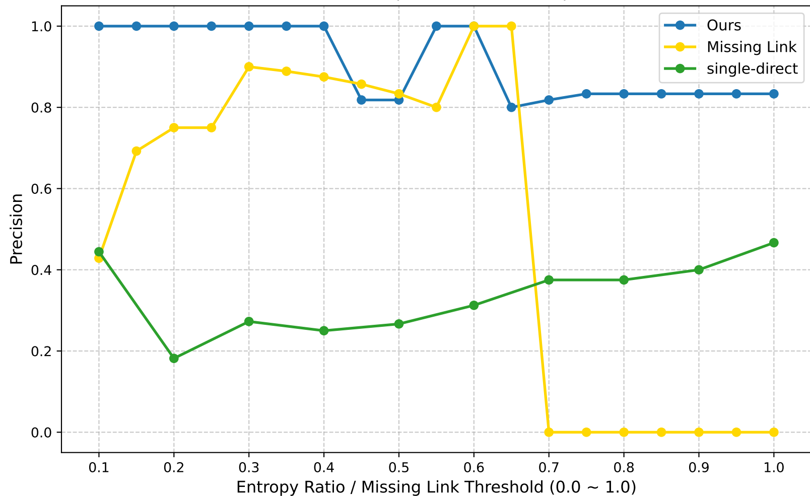
Precision (Global Round: 15)
