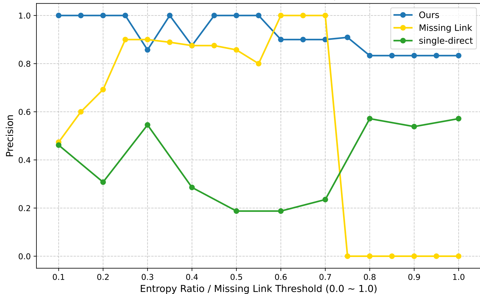
Precision (Global Round: 20)
