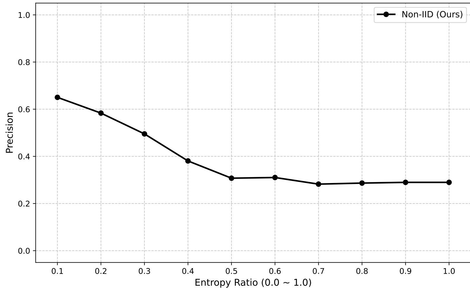
Precision (Global Round: 45)
