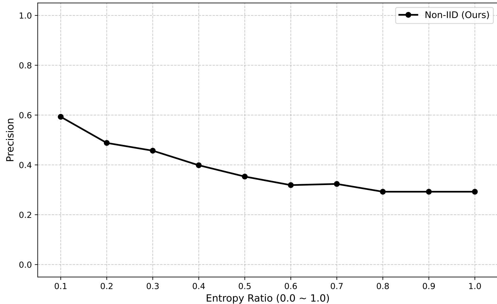
Precision (Global Round: 95)
