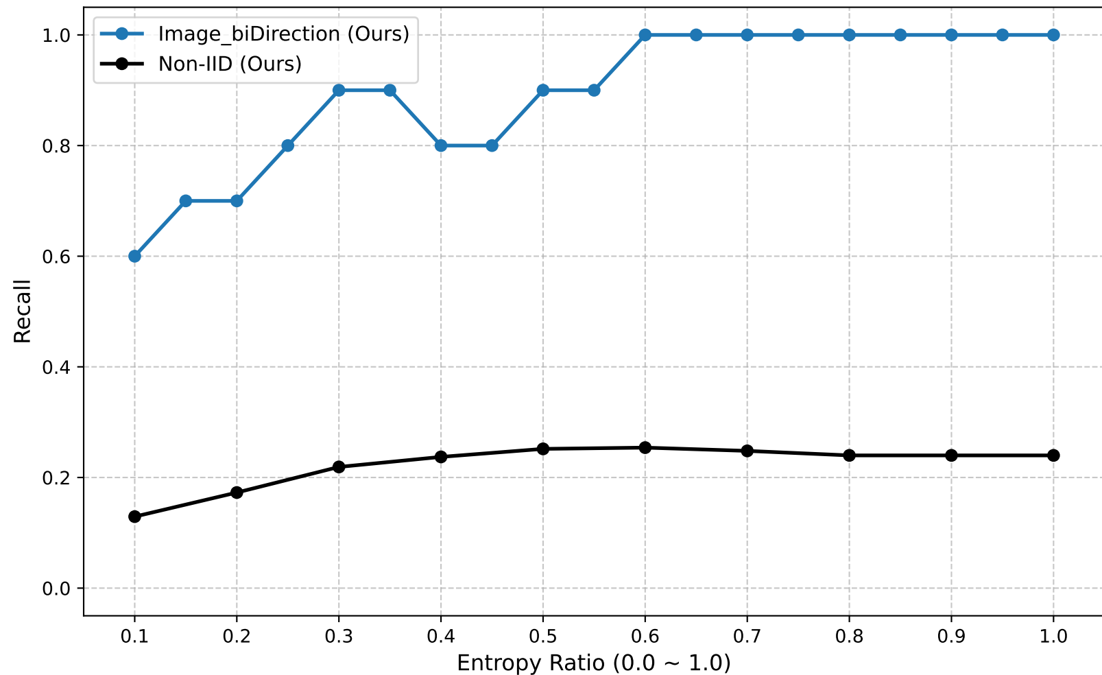
Recall (Global Round: 30)
