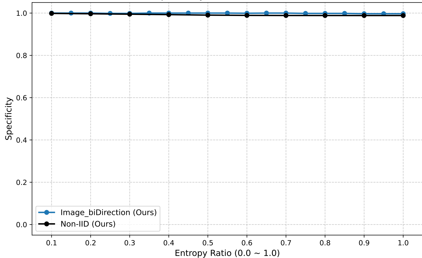
Specificity (Global Round: 35)
