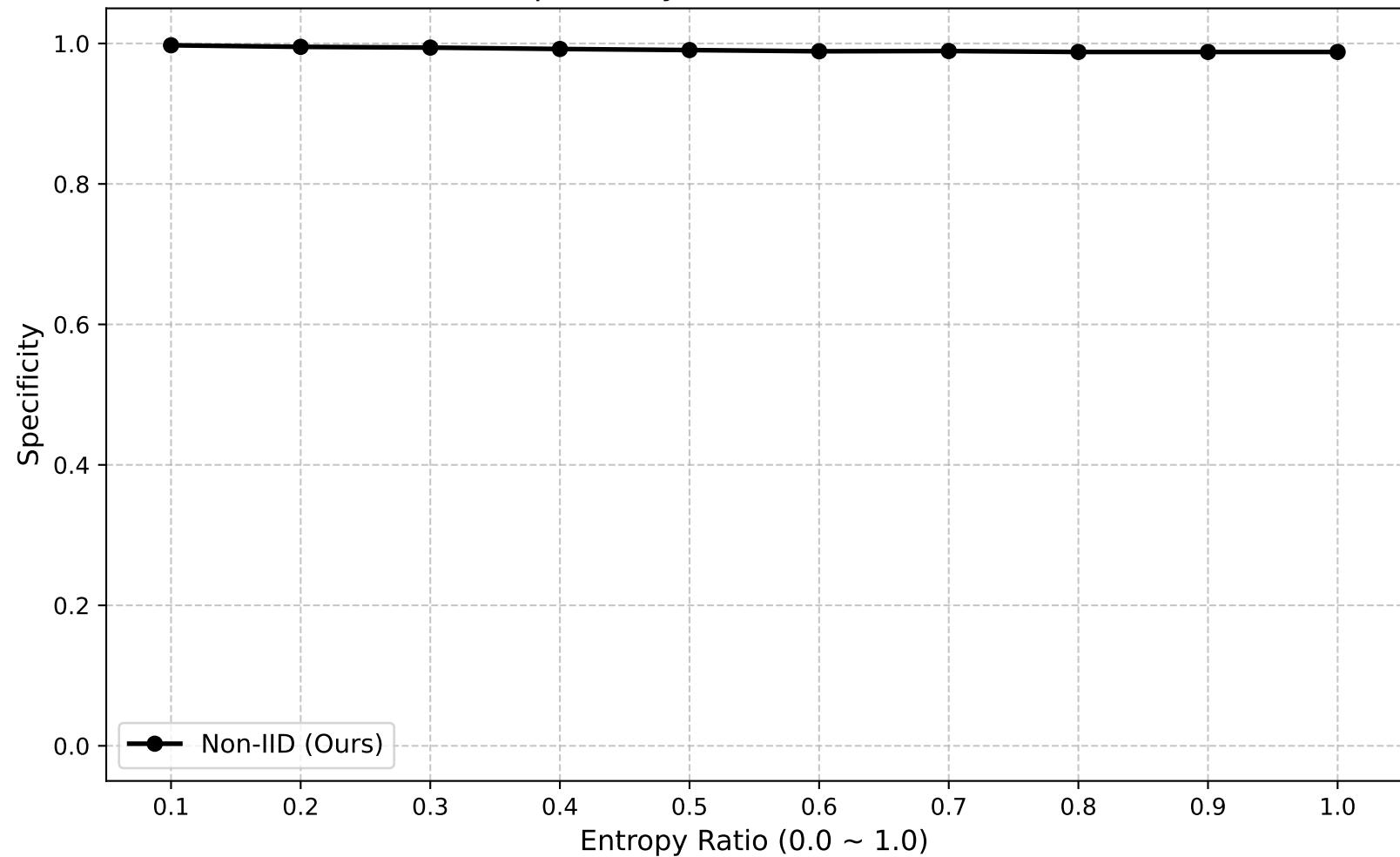
Specificity (Global Round: 95)
