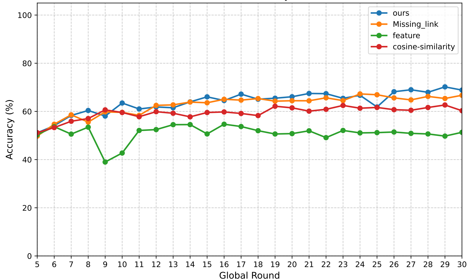
Global Model Accuracy on mix
